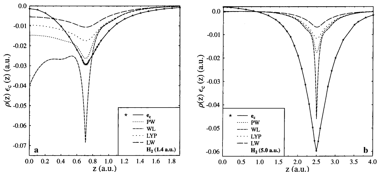
Figure 5. Correlation energy density in H_2 at R_e (a) and at R = 5.0 bohr (b) compared to model correlation energy densities. See caption to Figure 4. z is the coordinate along the internuclear axis; the bond midpoint is at z = 0.0 .
