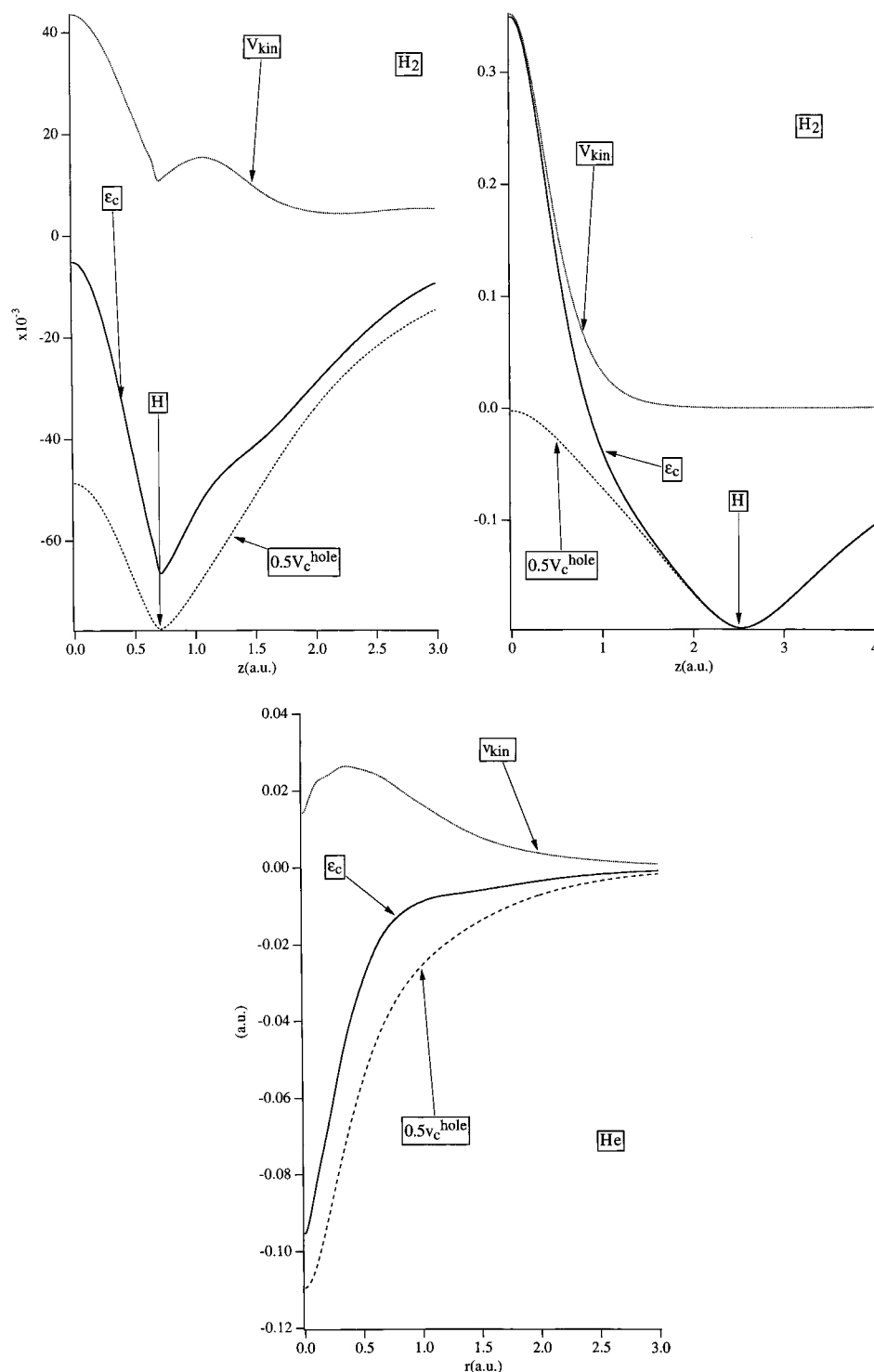
Figure 2. The correlation energy density \epsilon_c(\mathbf{r}) and its components v_{c,\text{kin}} ( = v_{\text{kin}} in these cases) in three cases: (a) plotted along the bond axis of H 2 at R(\text{H}-\text{H}) = 1.401 bohr ( R_e ) (the bond midpoint is at z = 0.0 ); (b) idem , at R(\text{H}-\text{H}) = 5.0 bohr; (c) for He.
