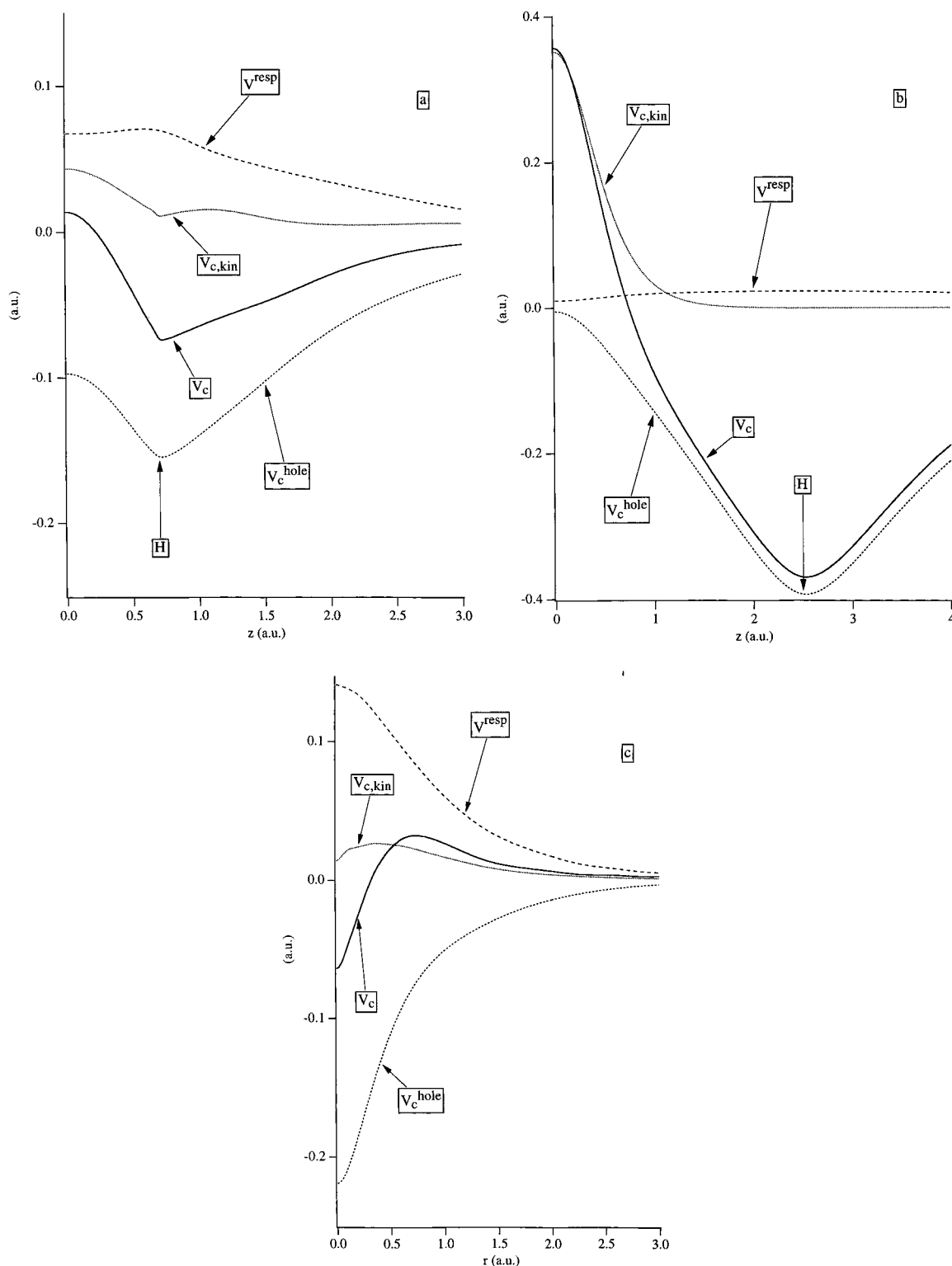
Figure 3. The correlation potential v_c and its components v_c^{\text{hole}} , v_{c,\text{kin}} ( = v_{\text{kin}} in this case), and v^{\text{resp}} ( = v^{N-1} in this case) for the cases: (a) plotted along the bond axis of \text{H}_2 at R(\text{H}-\text{H}) = 1.401 bohr ( R_e ) (the bond midpoint is at z = 0.0 ); (b) idem , at R(\text{H}-\text{H}) = 5.0 bohr; (c) for He.
