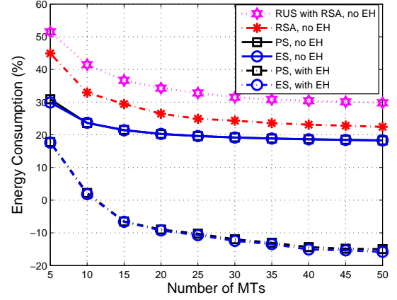
Figure 5. User energy consumption, with/without energy harvesting comparison
