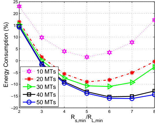
Figure 3. User energy consumption of CMC
