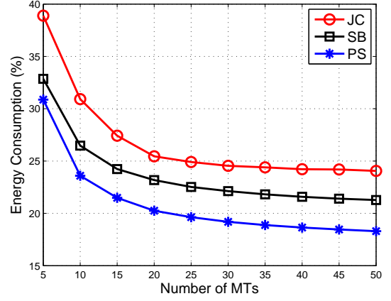
Figure 6. User Energy Consumption Performance Comparison
