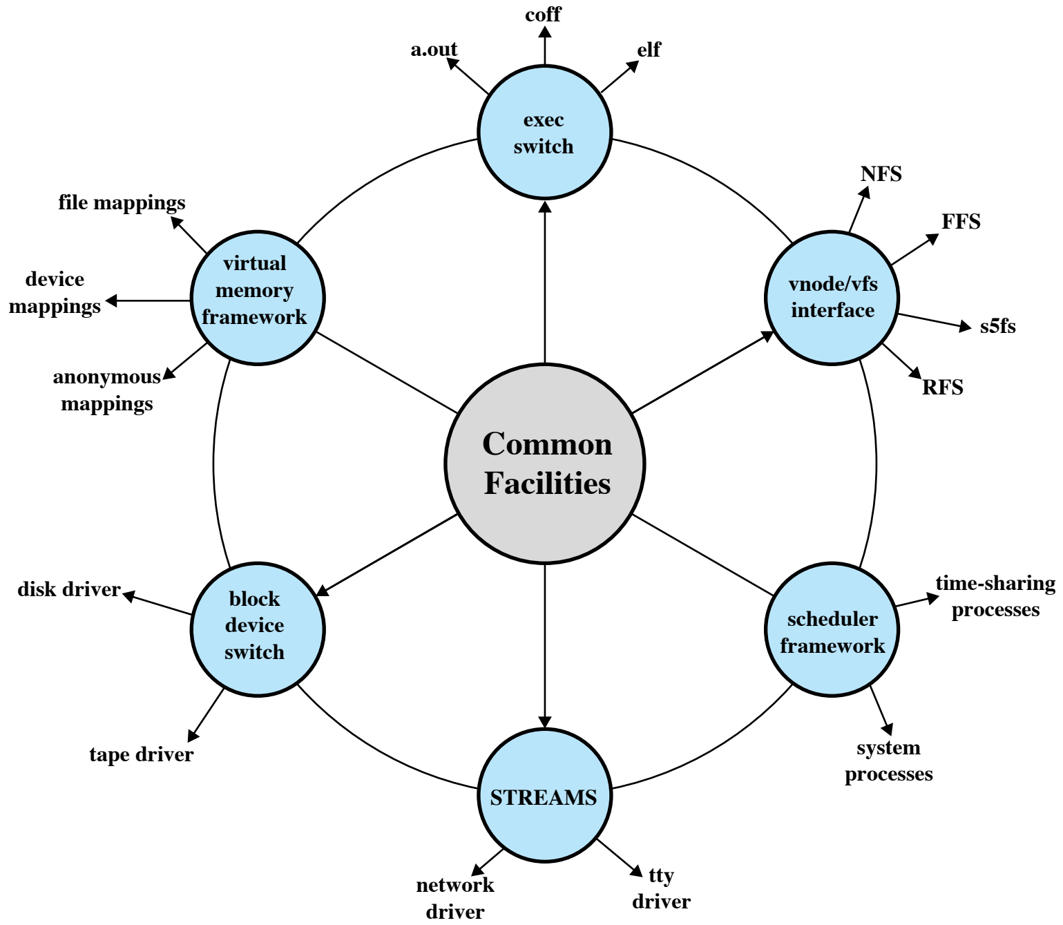
Figure 2.16 Modern UNIX Kernel [VAHA96]
