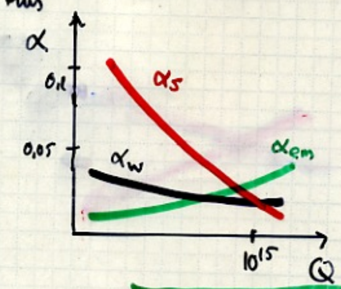
STANDARD MODEL
