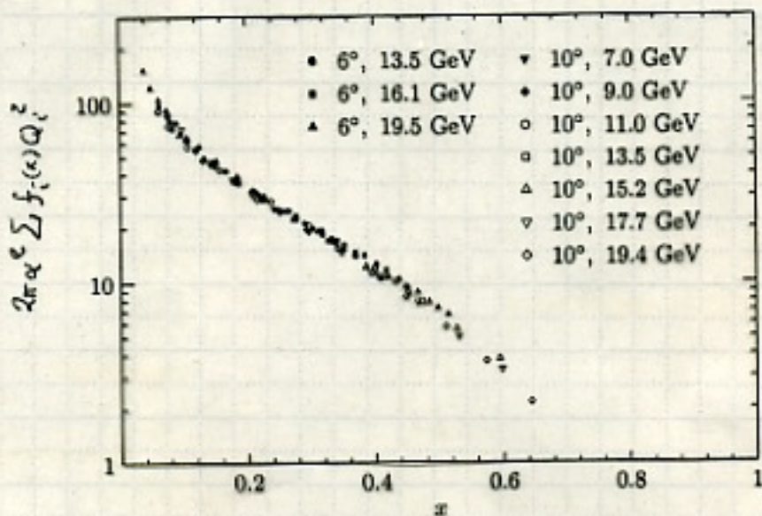
Figure 14.2. Test of Bjorken scaling using the e^-p deep inelastic scattering cross sections measured by the SLAC-MIT experiment, J. S. Poucher, et. al., Phys. Rev. Lett. 32 , 118 (1974). We plot d^2\sigma/dx dQ^2 divided by the factor (14.9) against x , for the various initial electron energies and scattering angles indicated. The data span the range 1 \text{ GeV}^2 < Q^2 < 8 \text{ GeV}^2 .
