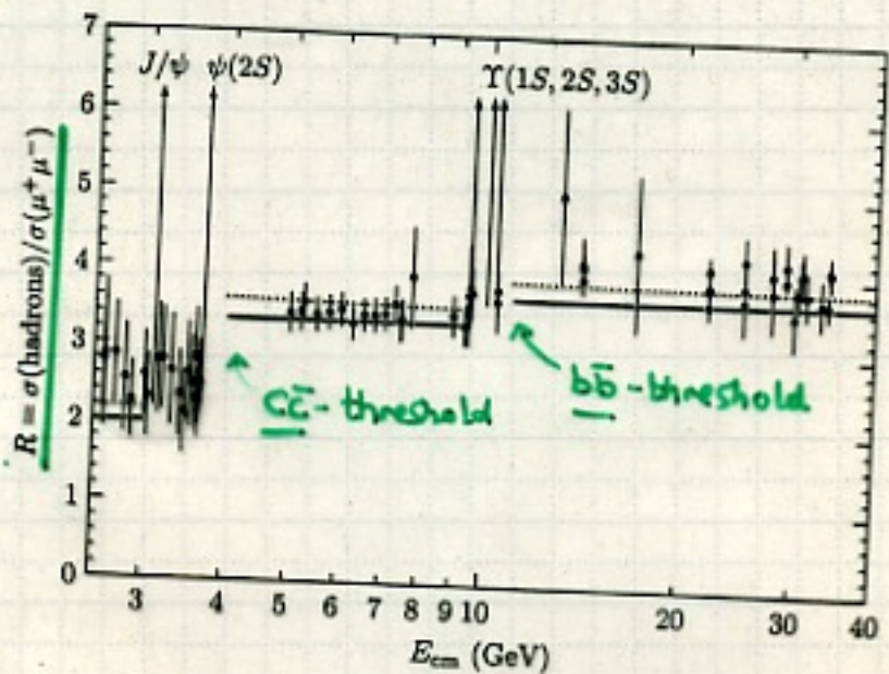
Figure 5.3. Experimental measurements of the total cross section for the reaction e^+e^- \rightarrow \text{hadrons} , from the data compilation of M. Swartz, Phys. Rev. D 53, 5268 (1996). Complete references to the various experiments are given there. The measurements are compared to theoretical predictions from Quantum Chromodynamics, as explained in the text. The solid line is the simple prediction (5.16).
