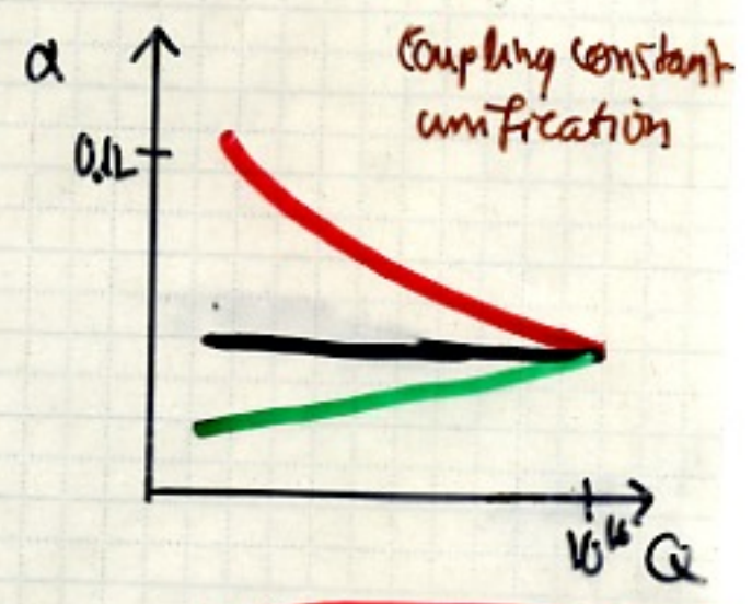
! SUPERSYMMETRY !
