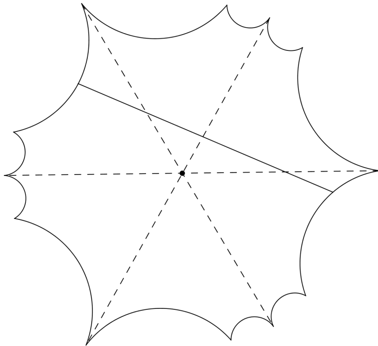
FIGURE 2. A conical domain \Omega with opening angle \pi/3 and a broken ray. See the proof of Proposition 6(1) for details.
