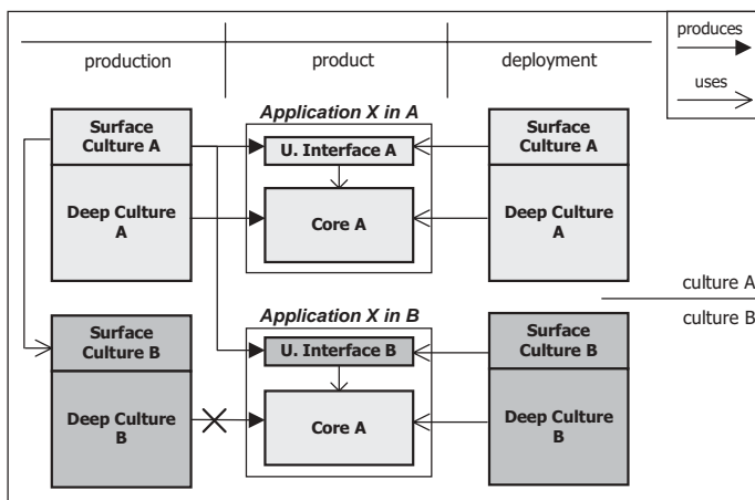
Figure 2. Internationalization of software produced in culture A
