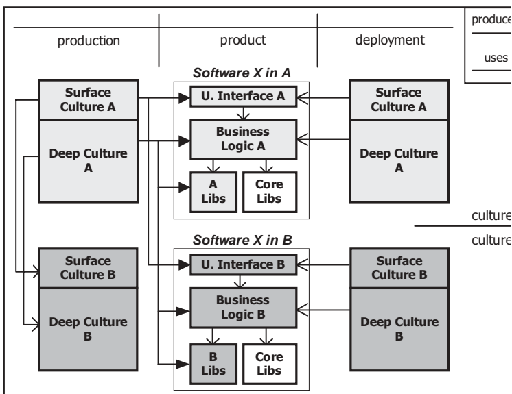
Figure 4. Culturalization of software produced in culture A
